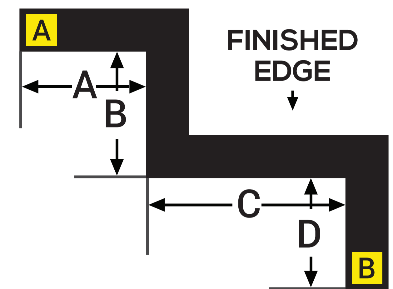
W PROFILE
